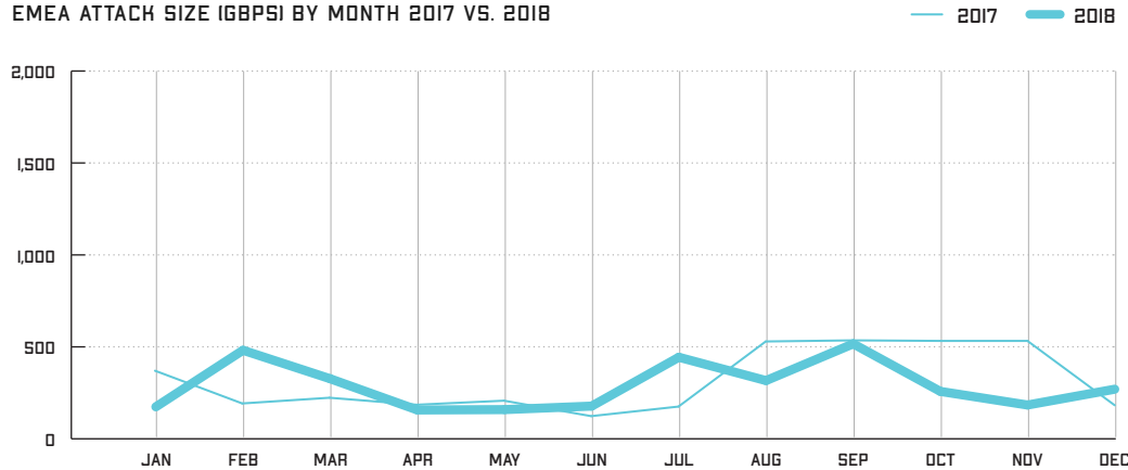
FIGURE 80 EMEA ATTACK SIZE (GBPS) BY MONTH 2017 VS. 2018
