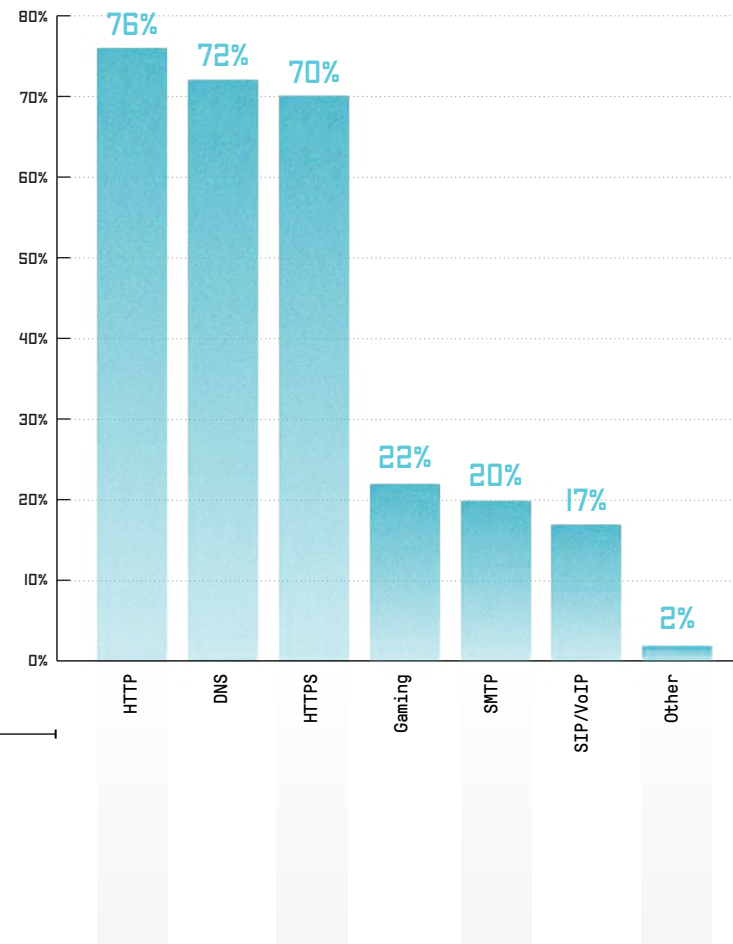
FIGURE 52 TARGETS OF APPLICATION-LAYER ATTACKS
